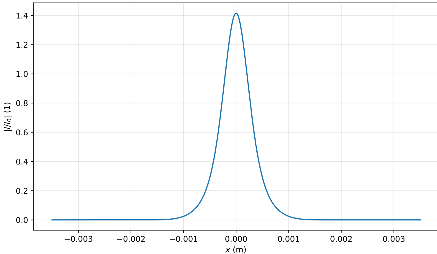
Intensity profile I(x, y = 0, z = 1.035m)/I_0 , P_{in}=0.9P_{cr} , artificial time
